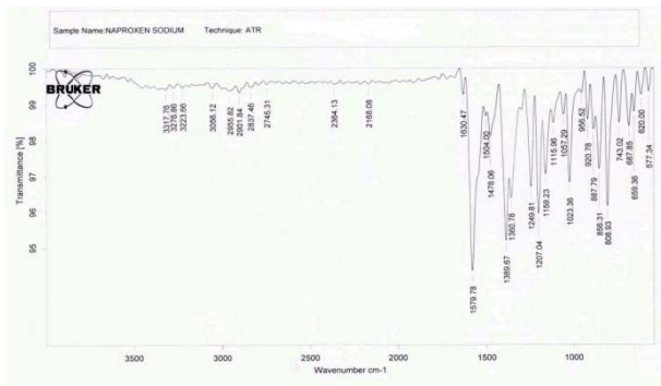
Figure 3: Infrared spectrum of Naproxen sodium
